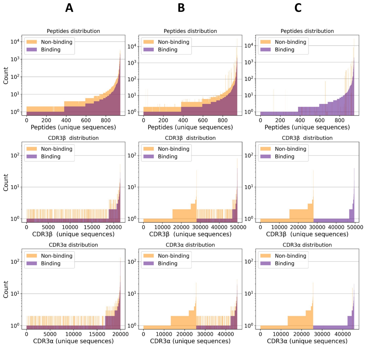
Figure 1. Class distribution of ( peptide; CDR3 \beta ; CDR3 \alpha ) samples. (A) Negative samples only include randomized negative samples (i.e. no negative assays). (B) Negative samples include negative assays and randomized negative samples. (C) Negative samples only include negative assays.
